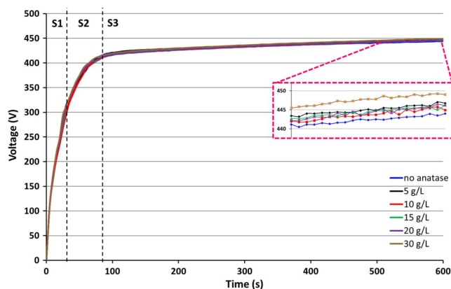
Figure 1. Voltage–time response for PEO processes with 0, 5, 10, 15, 20, and 30 g anatase particles addition.
