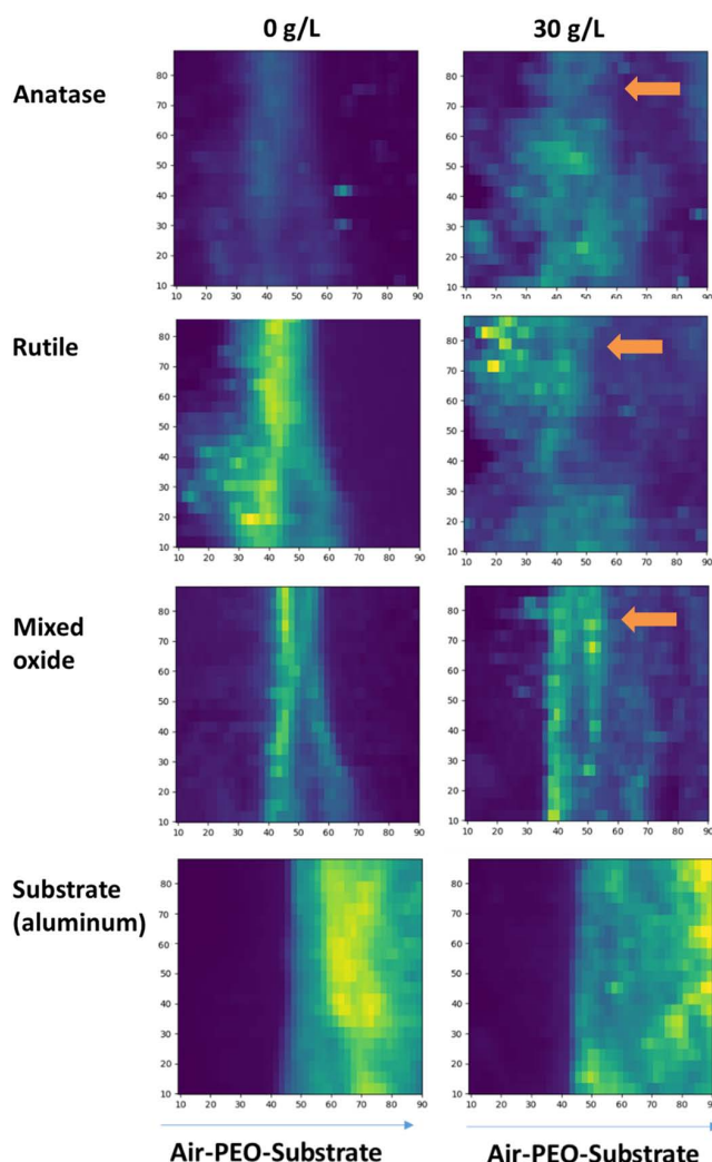
Figure 14. Distribution of the main phases in the coating and near substrate region determined by nanofocused high energy XRD. The orange arrow marks regions, where stronger discharge events appear to have taken place.
