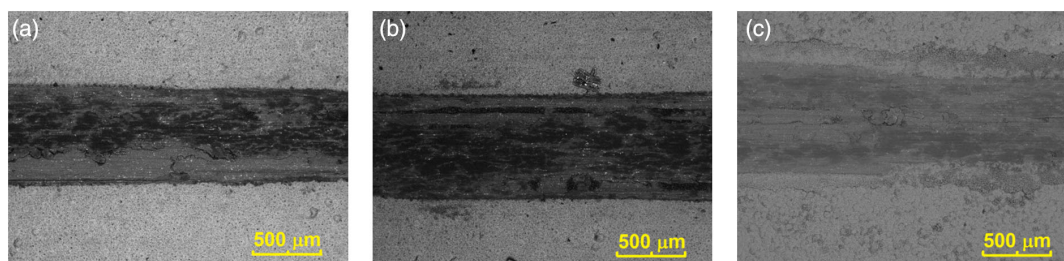
Figure 18. Wear tracks on samples that failed the wear test under different loads applied: a) 10 \text{ g L}^{-1} anatase—4 N; b) 15 \text{ g L}^{-1} anatase—5 N; and c) 30 \text{ g L}^{-1} anatase—6 N.
