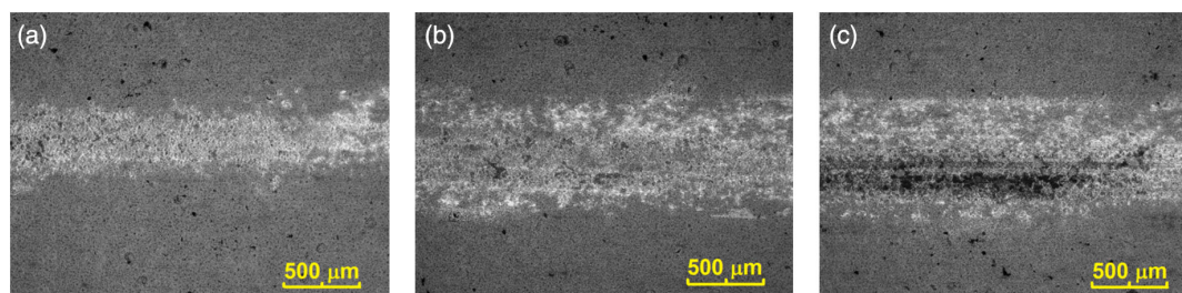
Figure 19. Wear tracks on samples that passed the wear test under different loads applied: a) 10 \text{ g L}^{-1} anatase—3 N; b) 15 \text{ g L}^{-1} anatase—4 N; and c) 20 \text{ g L}^{-1} anatase—5 N.
