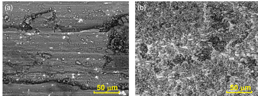
Figure 20. Cases of the PEO coating being a) completely removed and the substrate becoming exposed: 20 g L -1 anatase—5 N; and b) the coating remaining adherent leaving the substrate partially exposed: 15 g L -1 anatase—4 N.
