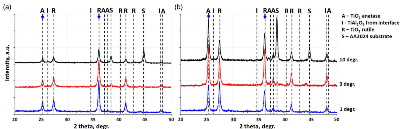
Figure 12. XRD patterns obtained at three different incident angles—a) standard electrolyte ( 0 \text{ g L}^{-1} ) and b) 30 \text{ g L}^{-1} anatase addition. Arrows are marking the rutile and anatase peaks used for calculating the rutile/anatase ratio.
