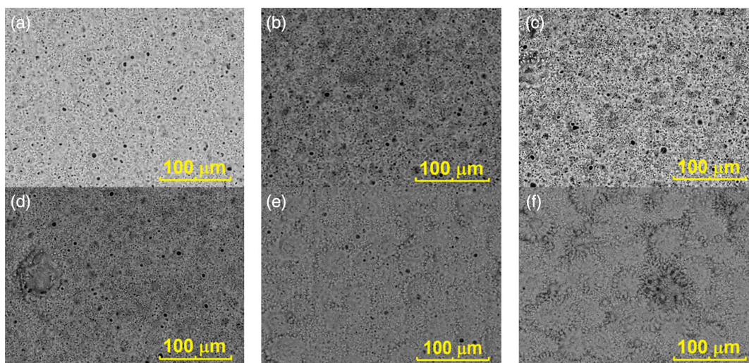
Figure 2. Surface morphology pictures of PEO coatings formed with different amounts of anatase particles addition, taken by SEM—a) 0 \text{ g L}^{-1} ; b) 5 \text{ g L}^{-1} ; c) 10 \text{ g L}^{-1} ; d) 15 \text{ g L}^{-1} ; e) 20 \text{ g L}^{-1} ; and f) 30 \text{ g L}^{-1} .
