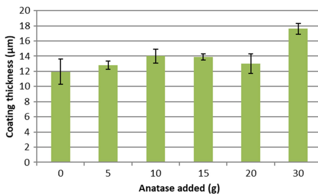
Figure 7. Coating thickness as function of anatase concentration in electrolyte (0 till 30 g \text{L}^{-1} ) measured by thickness gauge.
