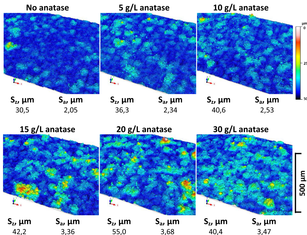
Figure 4. Surface morphology as measured by laser scanning microscope and corresponding height parameters S_z and S_a after 10 min PEO processing as a function of anatase content in the electrolyte.
