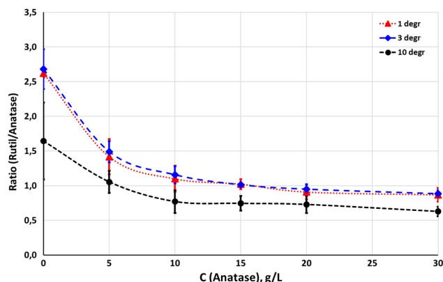
Figure 13. Figure 13. Rutile to anatase ratio as a function of the amount of anatase particles addition to the electrolyte, calculated from the XRD measurements using the highest intensities of rutile (101) and anatase (101) peaks (at around 36^\circ [39] and 25.2^\circ [40], respectively).
