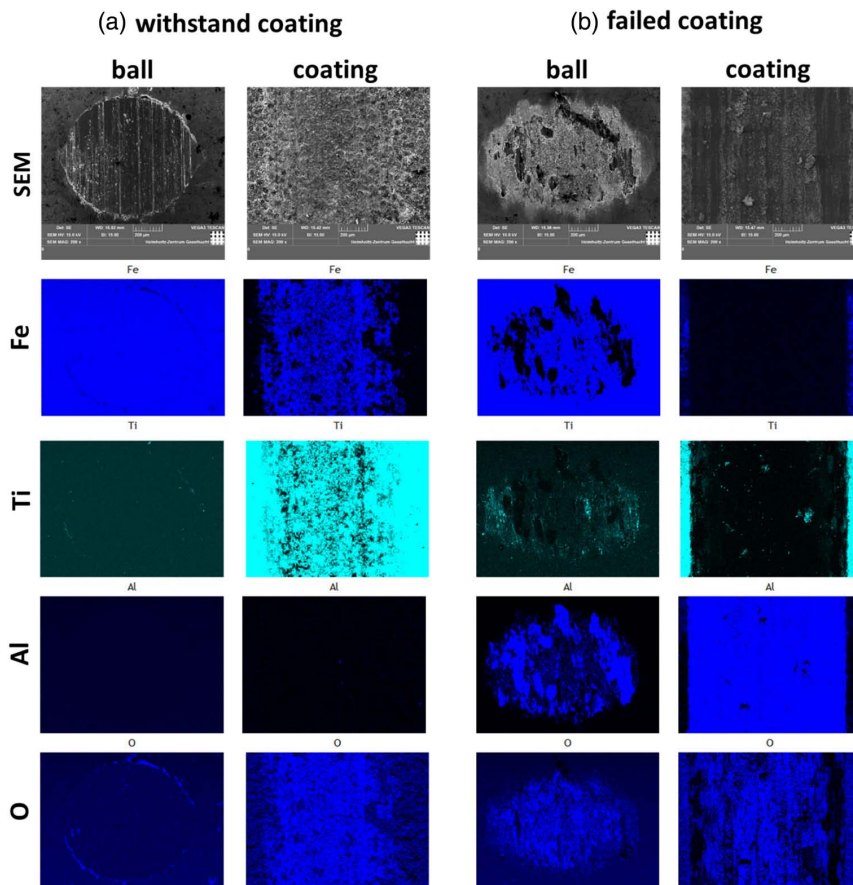
Figure 21. Elemental distribution maps after the wear test in the case of withstand and failed coatings. PEO treatment in the presence of 15 g L -1 anatase is selected as representative.
